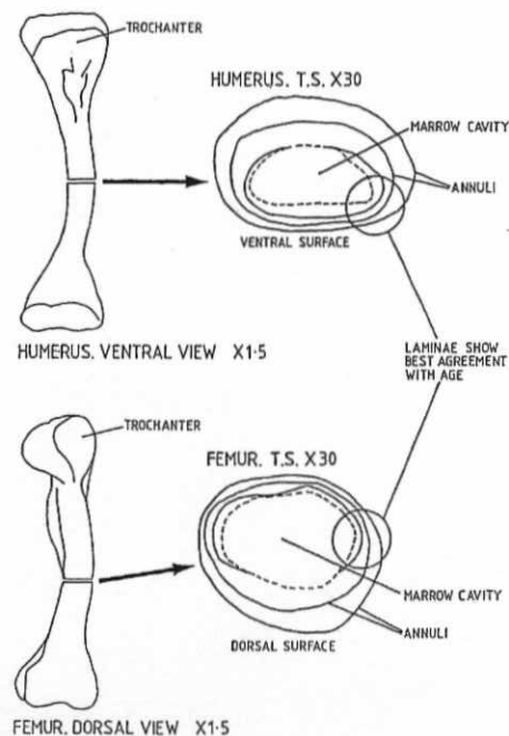
Fig. 5. Cross-sections taken mid-diaphysis from the long bones of a young Nile crocodile. Growth is unequal and the marrow activity is drifting towards the dorsal surface. Lateral laminae show the best agreement with age.
