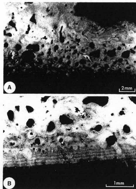
Fig. 7. Thin section of the neck osteoderm of "Beadle" aged 45 years and 10 months. The internal reworking, expansive vascular canals and narrow ventral laminar band, shown in A, are typical of a breeding female. 18 distinct annuli are arrowed in enlargement B.
