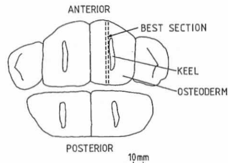
Fig. 2. The dorsal neck osteoderms of a crocodile showing the most useful section for ageing a live animal.
